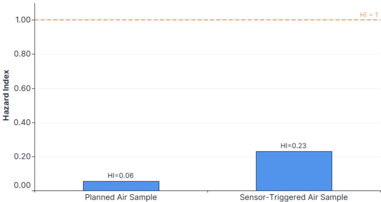
Figure 5 Hazard Indices at the CCND CM2 – Suncor Business Center for Planned (August 27, 2025) and Sensor-Triggered (July 21, 2025) Air Samples
